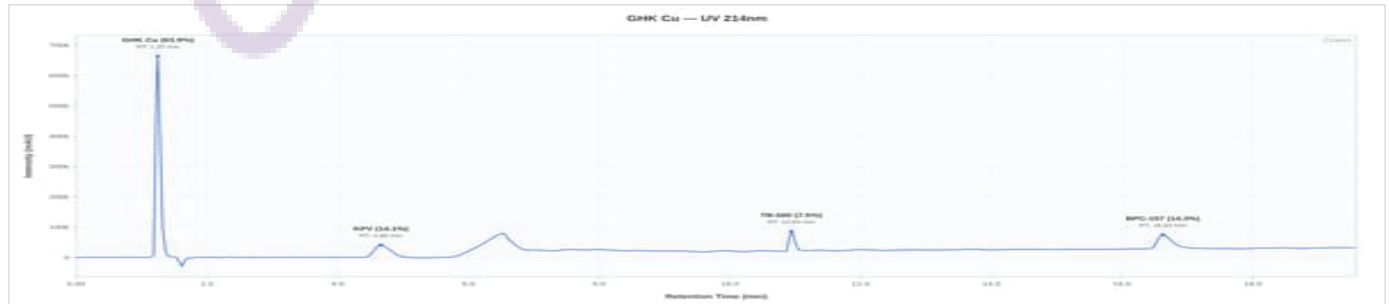
KLOW 50/10/10/10 - Klow05102026: UV Chromatogram
