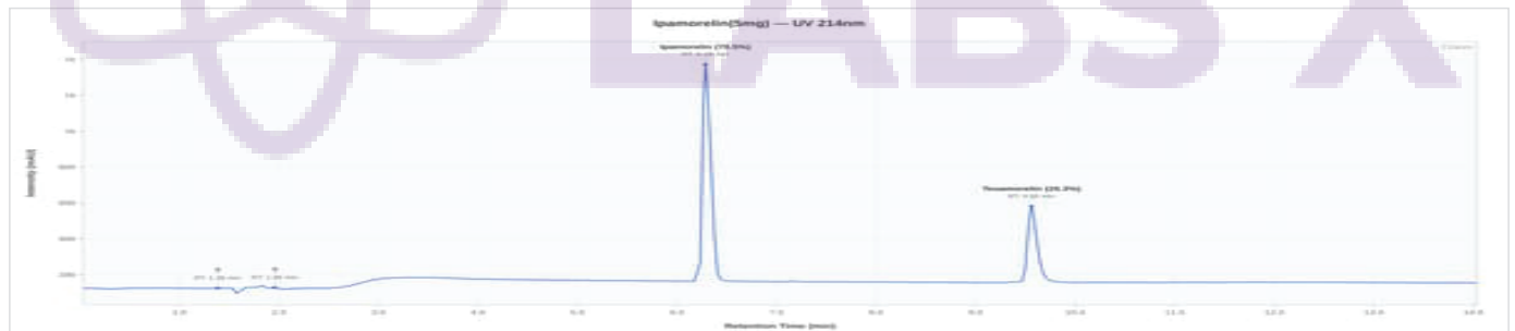
Tesamorelin / Ipamorelin 15mg - Teslpa06122026: UV Chromatogram
